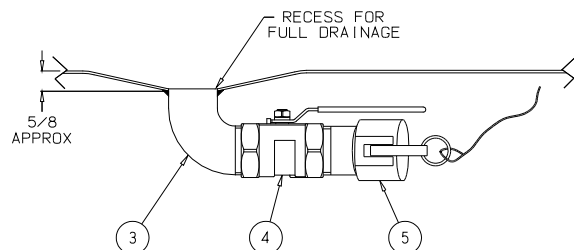
VALVE ASSEMBLY DETAIL SCALE: NONE
